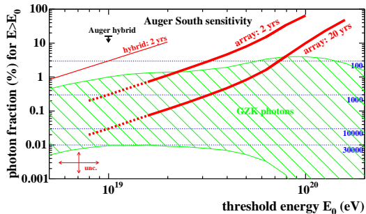
Figure 4: Fraction of photons in the integral cosmic-ray flux as a function of the threshold energy. The GZK photon prediction is taken from [18]. Photon fractions of 0.1-0.01% were obtained in recent calculations [19, 20]. For reference, the limit from Auger hybrid data [16], obtained with 29 events, is shown. Numbers on the right-hand side give the minimum number of events required to place a 95% c.l. limit at the level indicated by the horizontal lines. An estimate for the sensitivity (see [4] for details) of the array of the southern Auger Observatory is shown for two and twenty years of operation based on the Auger spectrum [21] and assuming a flux suppression above E_{\text{GZK}} . Also shown is the estimated sensitivity using hybrid data, which are less numerous but reach to smaller energy. The uncertainty of the sensitivity estimates is indicated at the lower left corner. At around 10^{19} eV (dashed lines), additional threshold effects may become increasingly important for the array. If complemented by an extended northern array, a sensitivity level of below 0.1% can be reached within a few years of operation.
