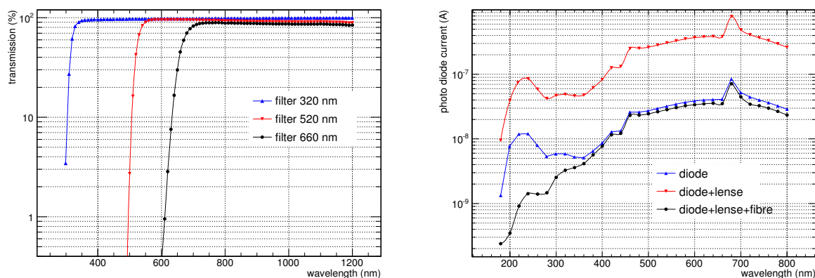
Figure A.3 – Left: Transmission of the order sorting filters as measured with a Varian Cary 500 spectrophotometer. Right: Photodiode current as function of wavelength with and without optical fibre. The attenuating behaviour of the fibre below 350 nm can be seen.
