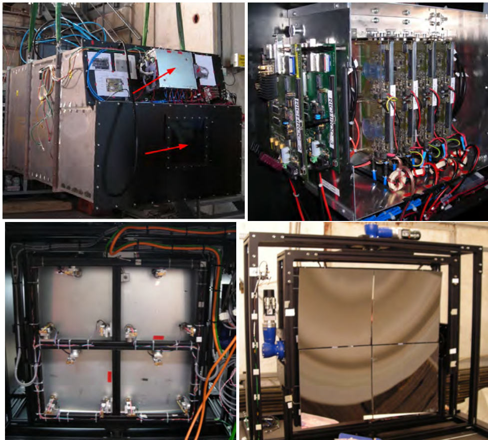
Figure 5.2 – Top: CBM-RICH prototype from the front. The quadratic beam entrance window and the camera housing are marked with arrows (left). Readout electronics (right). Bottom: Mirror tiles mounted on the rotatable frame from back (left) and front (right).
