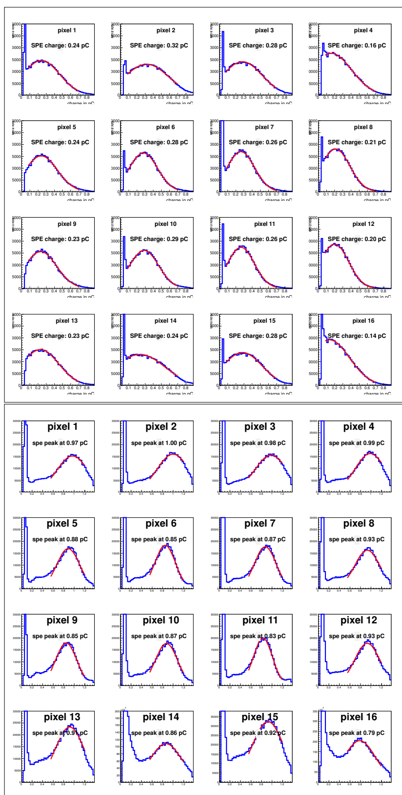
Figure C.5 – Single photoelectron spectra two R11265-103-M16. One average tube is shown on the top (ZN0733) and one with very high gain at the bottom (ZN0593). The scale on the x -axis spreads from 0 pC to 0.9 pC on top and from 0 pC to 1.4 pC at the bottom.
