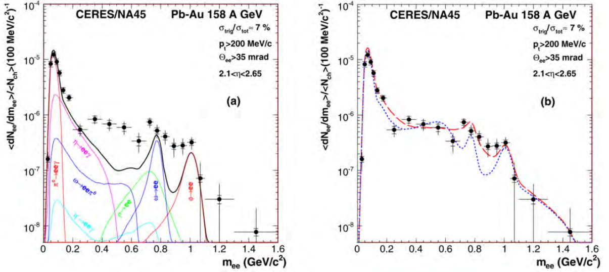
Figure 2.4 – Invariant mass spectrum of di-electrons measured by the CERES experiment in the range from 0 \text{GeV}/c^2 to 1.6 \text{GeV}/c^2 for Pb+Au collisions at the energy of 158 A GeV. Left: Comparison of the measured di-electron yield to the hadronic cocktail (solid line). An excess in the data over the cocktail can be observed in the range from 0.2 \text{GeV}/c^2 to 0.7 \text{GeV}/c^2 . Right: Comparison of data with calculations including a dropping \rho^0 mass (dotted line) and a broadening of the \rho^0 spectral function (dashed line). It can be seen that the latter is in better agreement with the data. Figure taken from [48].
