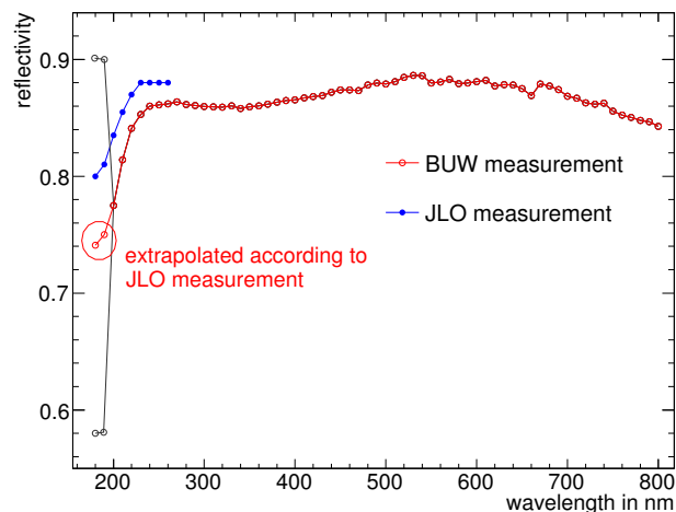
Figure 6.5 – Wavelength dependent mirror reflectivity as measured at BUW and by the manufacturer JLO. The BUW measurement shows the average reflectivity of the four mirror tiles mounted in the prototype (open red symbols). The JLO data shows the results from a measurement of another mirror tile of the same type (filled blue symbols). Since the BUW measurement only goes down to 200 nm, the two data points at 180 nm and 190 nm are extrapolated. They are calculated by subtracting from the JLO data points the difference between JLO and BUW data at 200 nm. The grey symbols show an assumed reflectivity of 90 % and 58 % in order to study the influence on the hit multiplicity. A full MC simulation of the prototype reveals that the hit multiplicity varies only by \pm 0.1 photoelectrons per electron ring when assuming a reflectivity of (74 \pm 16) \% with 74 % being the value implemented in RICHglassJLO at 200 nm.
